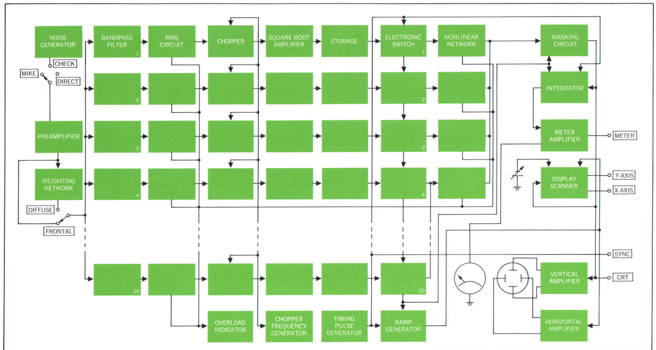
Fig. 4. Model 8051A Loudness Analyzer splits frequency range from 45 Hz to 14 kHz into 20 bands which approximate the ear's critical bands. Signals in each band are scanned sequentially after processing to reproduce Zwicker diagrams on CRT or X-Y recorder.
